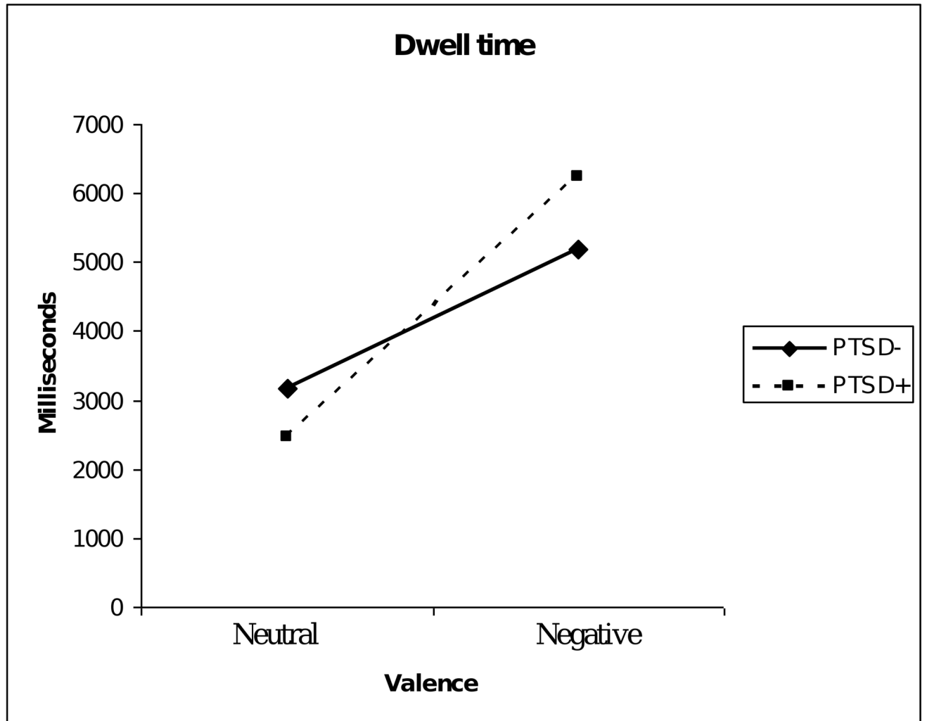
Figure 3. Dwell Time as a function of Valence and PTSD symptom reports
