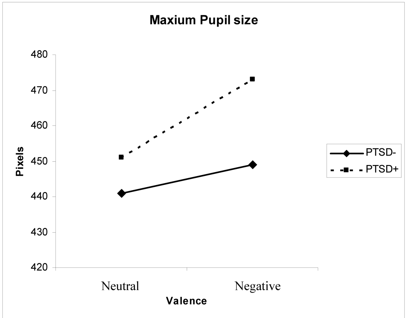
Figure 2. Maximum pupil size as a function and Valence and PTSD status.
